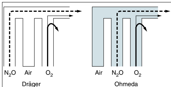
Fig. 15.4 Oxygen flow tube leak. An oxygen flow tube leak can produce a hypoxic mixture regardless of the flow tube arrangement. (From Brockwell RC. Inhaled anesthetic delivery systems. In Miller RD, ed. Miller's Anesthesia . 7th ed. Philadelphia: Churchill Livingstone; 2010:680, used with permission.)
