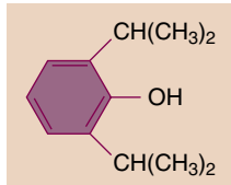
Fig. 8.1 Chemical structure of 2,6-diisopropylphenol (propofol).
