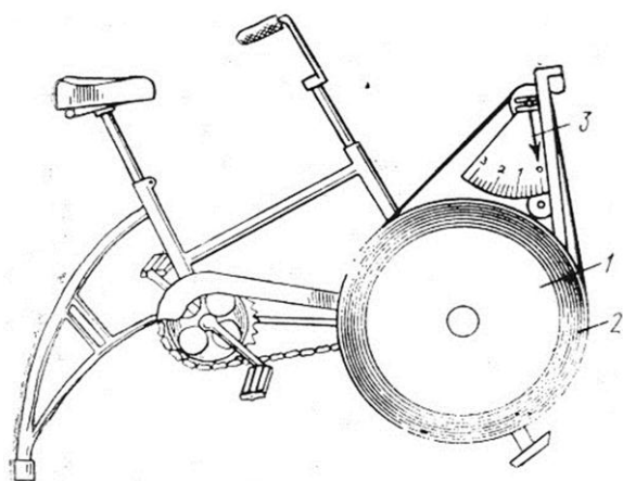
1.15-rasm Veloergometr
