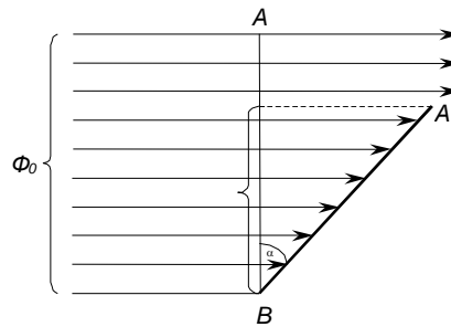
7.11-rasm. Yorug`lik oqimi ( \Phi )ning sirtga burchak ostida tushishi
