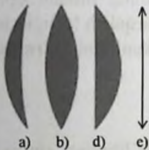
7.4-rasm. Yig'uvchi linza
