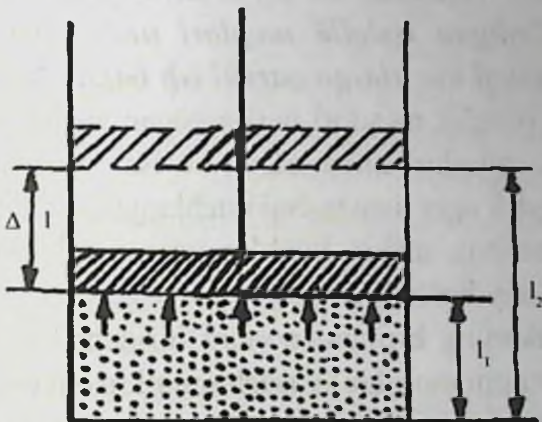
4.2-rasm. Gaz hajmining o'zgarishida gaz bajargan ishi
