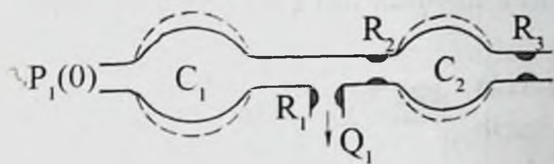
3.4-rasm. Roston modeli
