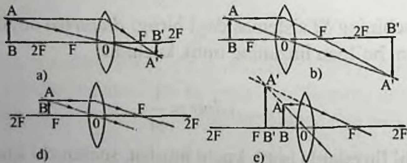
7.8-rasm. Qavariq linzada tasvirning hosil bo`lishi
