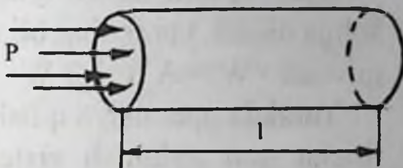
3.9-rasm. Qonning zarb hajmini silindri ko'rinishi
