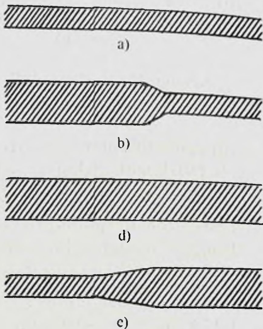
3.6-rasm. Arteriyaning yon tomonidan sxematik ko'rinishi
