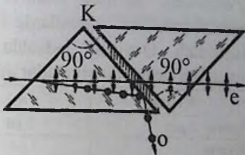
7.32-rasm. Nikol prizmasi
