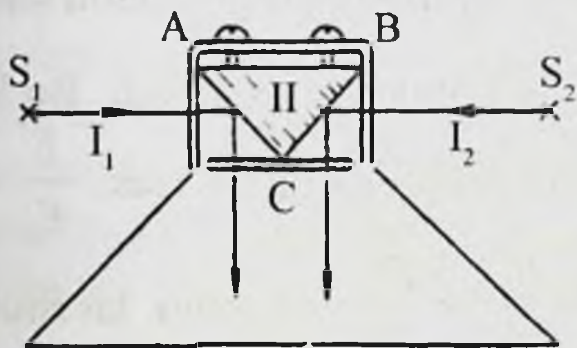
7.12-rasm. Eng sodda fotometrning tuzilishi
