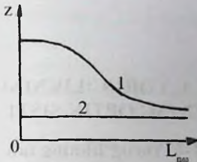
6.5-rasm. To‘qima impedansining chastotaviy bog‘lanishi.
