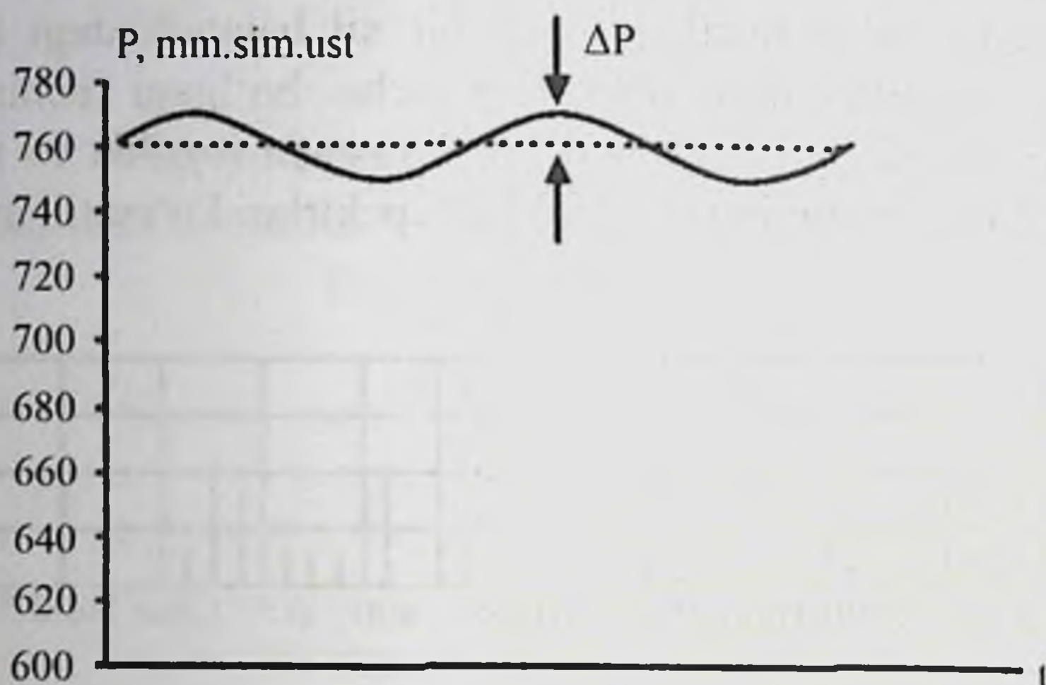
5.2-rasm. Muhitda tovush tarqalishida bosimning o'zgarishi.
