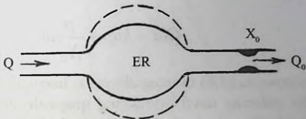
3.1-rasm. Qon aylanish sistemasining elastik rezervuar kabi modellashtirilishi
