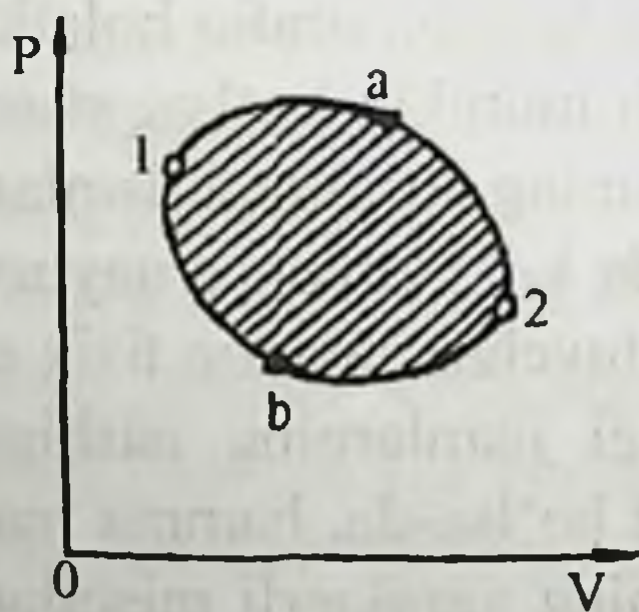
4.8-rasm. Teskari sikl (qaytmas jarayon)
