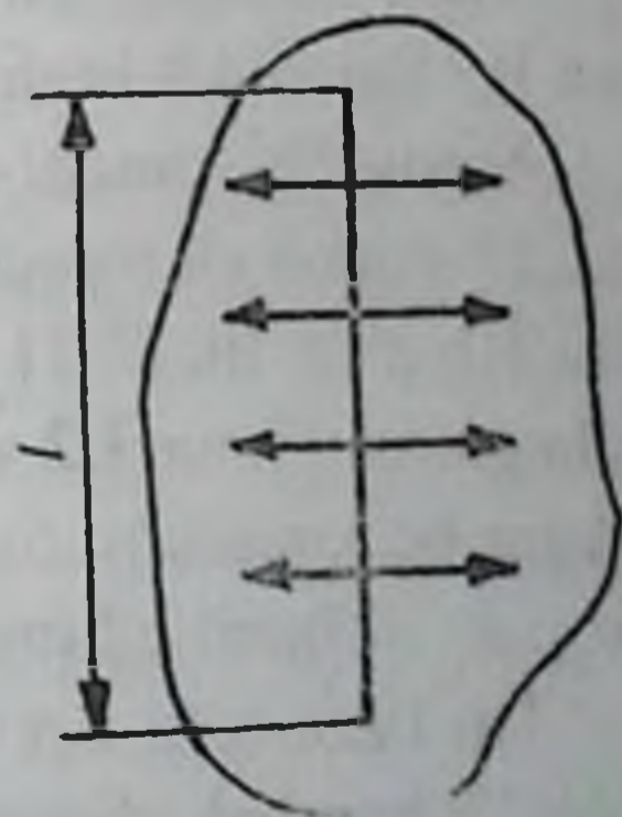
2.10-rasm. Sirt taranglik kuchini hosil bolishi
