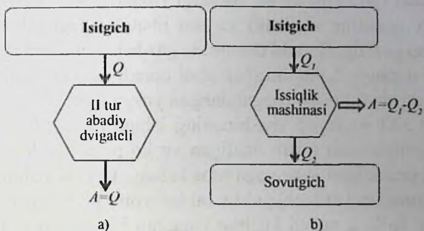
4.6-rasm. Ideal (a) va real (b) issiqlik mashinalari ish prinsipi
